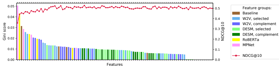
Fig. 1: An example of feature importance and performance analysis for a Learning-to-Rank approach.
